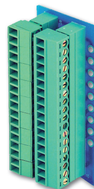
TB18 Pluggable Terminal Block
